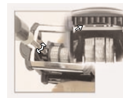
Adjusting the date bands to the exact height of the textplate:
